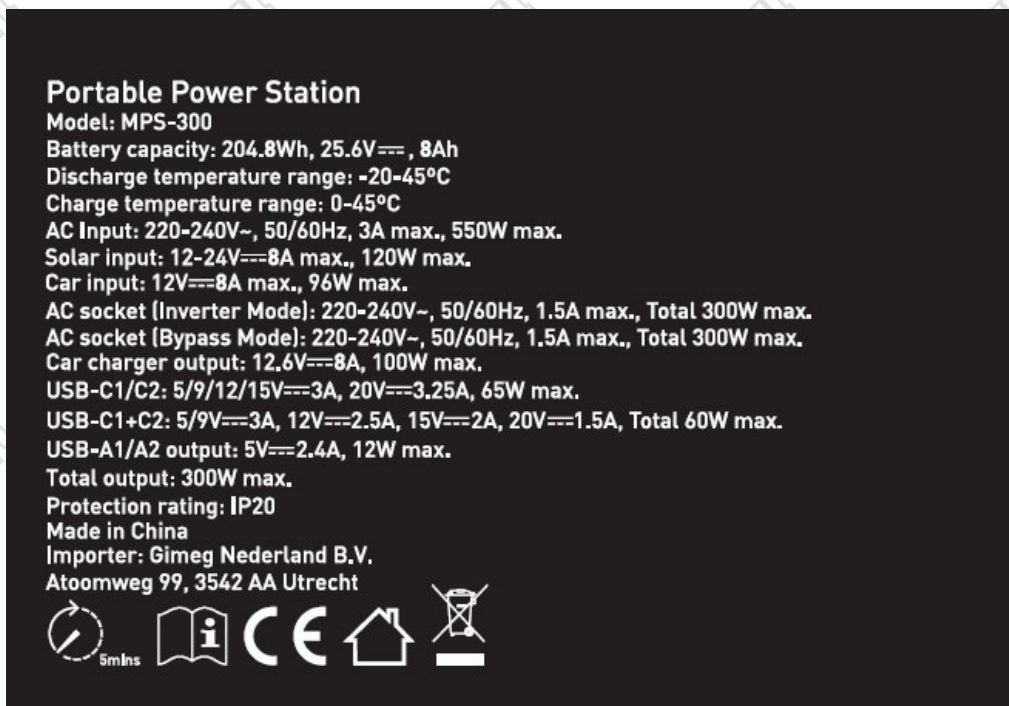
Figure 4 Battery Label
